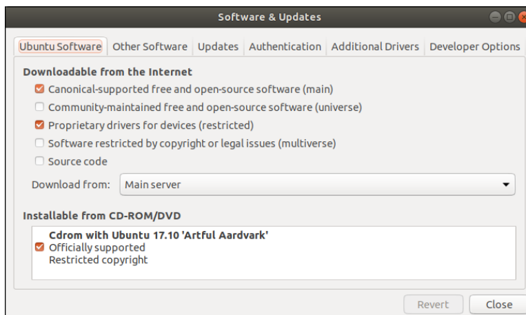
FIGURE 3-6: Software & Updates.
