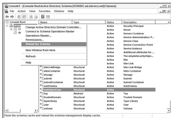
Figure 13-16: Reloading the schema cache.
