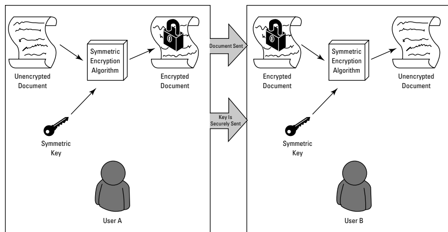
Figure 10-7: Symmetric encryption.
